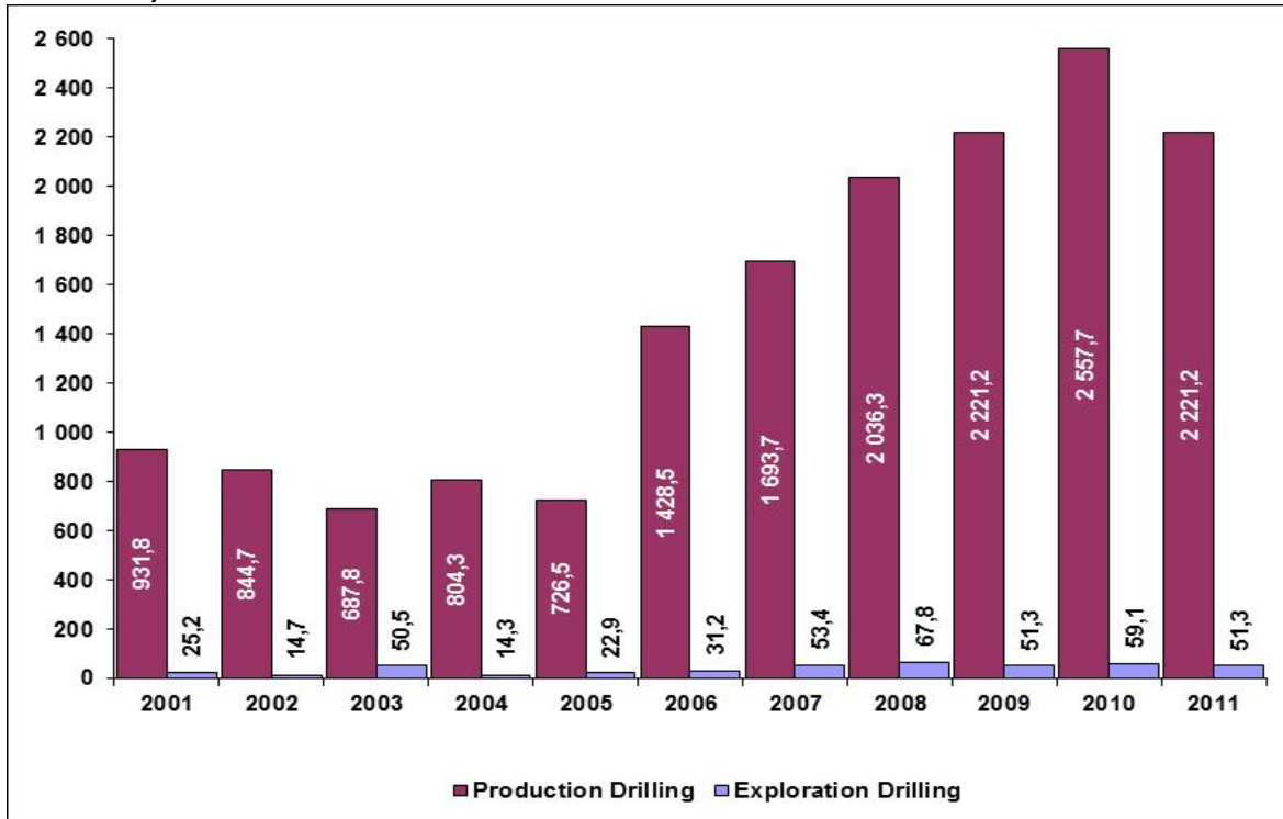
Figure 3.2.6. Gazprom Neft production and exploration drilling in 2001-2011 (thousands of meters)
